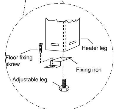
Fixing of the heater to the floor. NOTE! Fixing from two (2) of the legs.
